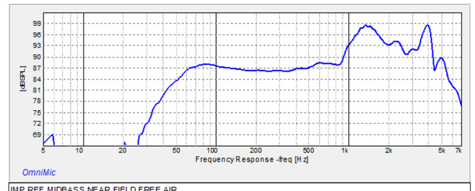
IMP REF MIDBASS NEAR FIELD FREE AIR
