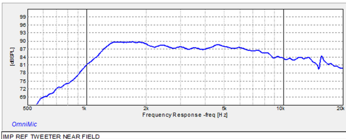
IMP REF TWEETER NEAR FIELD
